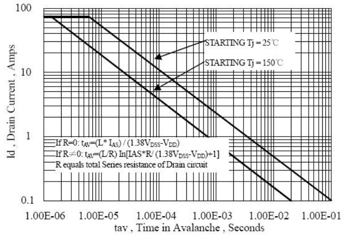
Figure 16 Unclamped Inductive Switching Capability
