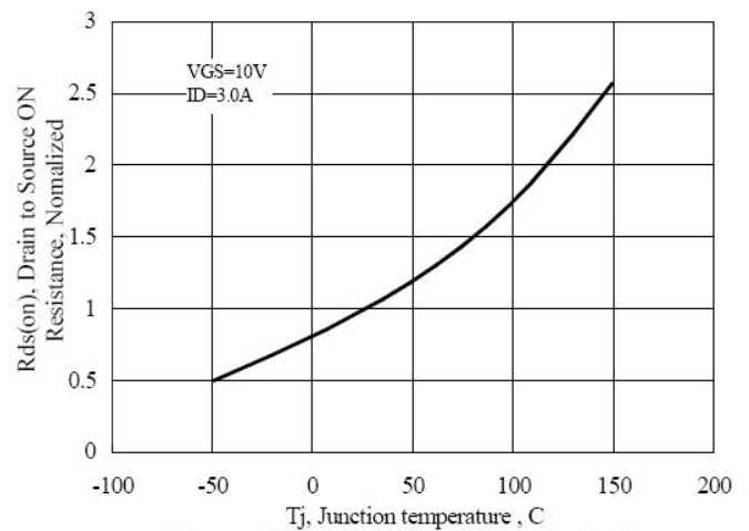
Figure 10 Typical Drain to Source on Resistance
